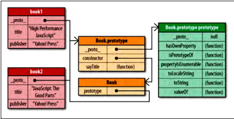
Figure 2-10. Prototype chains
