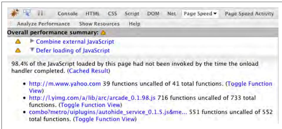
Figure 10-12. Page Speed deferrable JavaScript summary
