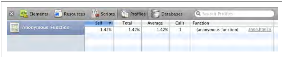
Figure 10-7. Web Inspector Profile panel showing anonymous function
