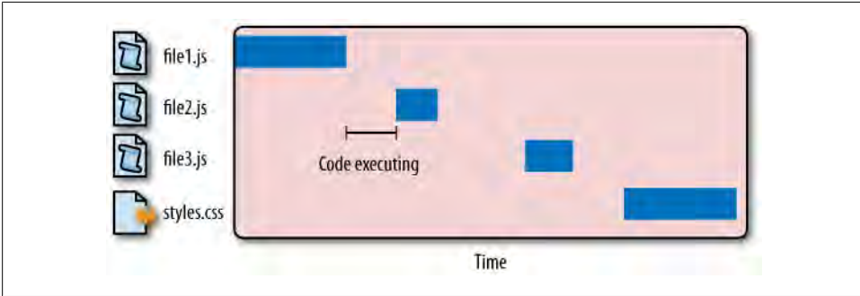
Figure 1-1. JavaScript code execution blocks other file downloads
