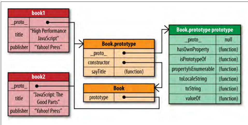
Figure 2-10. Prototype chains
