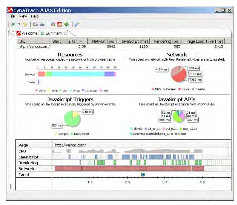
Figure 10-19. dynaTrace Ajax Edition: Summary report
